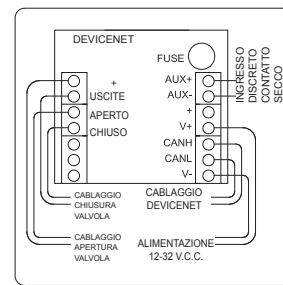
DeviceNet
